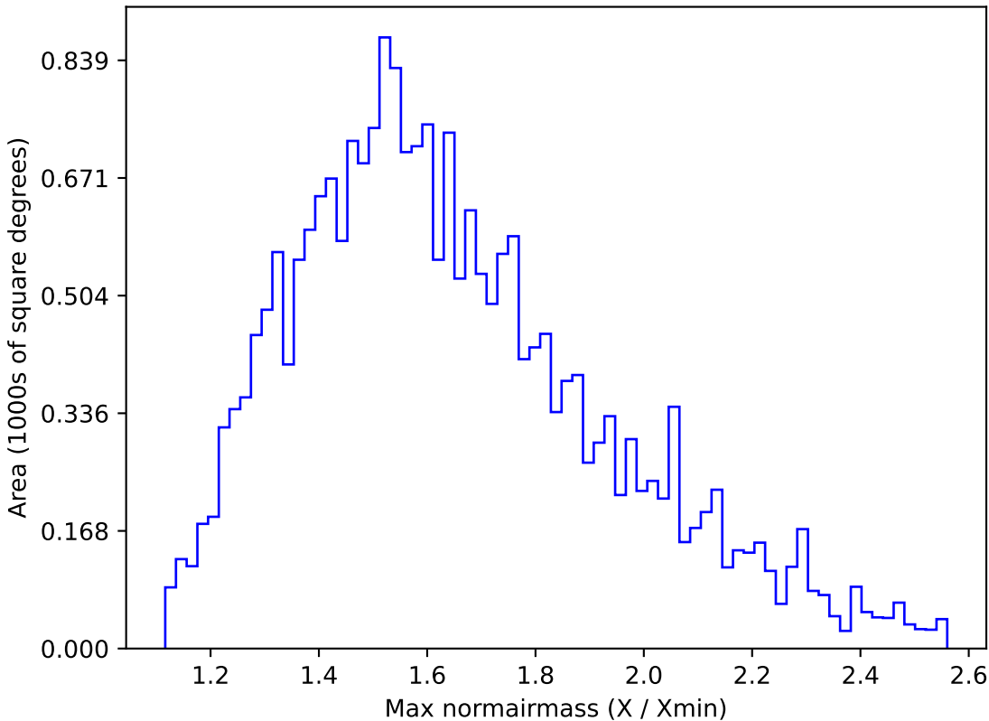
smc_lmc_v3.3_10yrs All sky u band: Max normairmass
