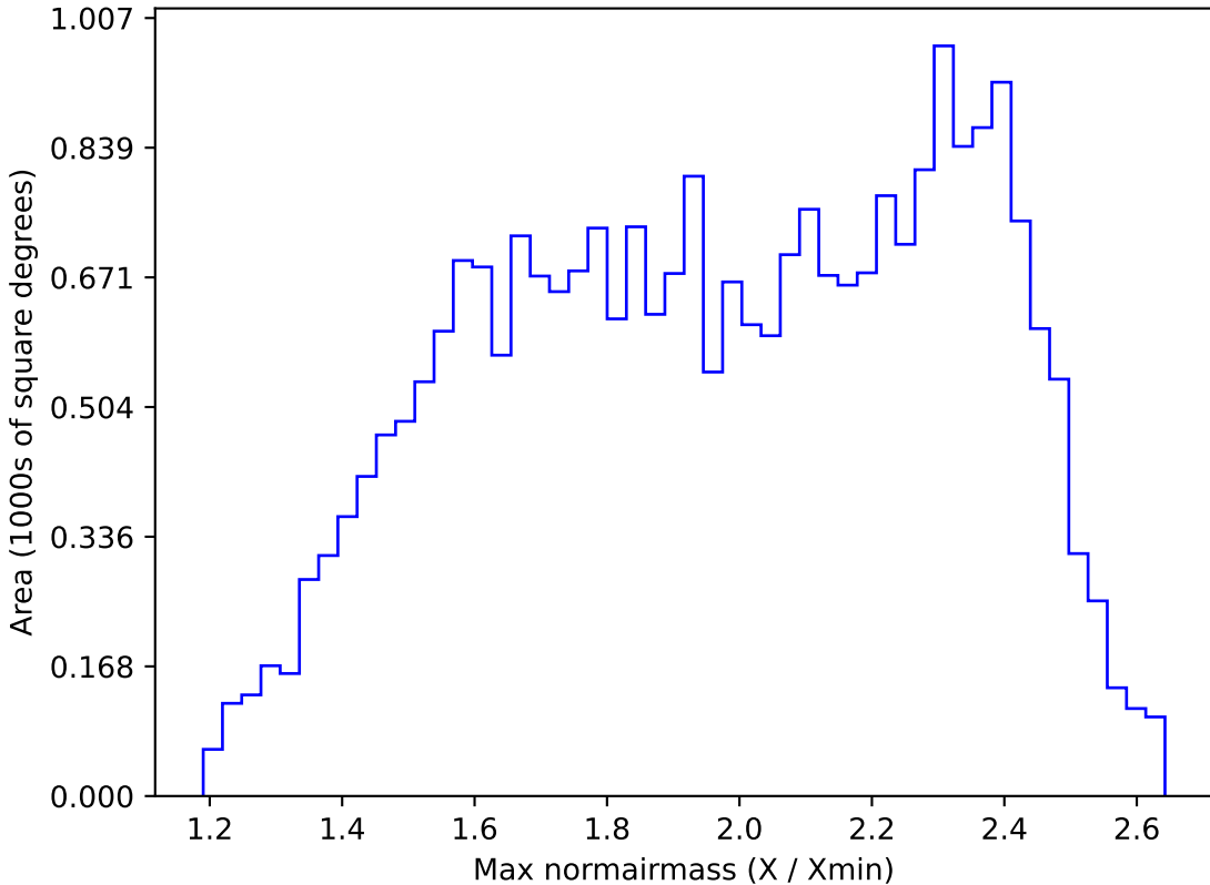
smc_lmc_v3.3_10yrs All sky r band: Max normairmass
