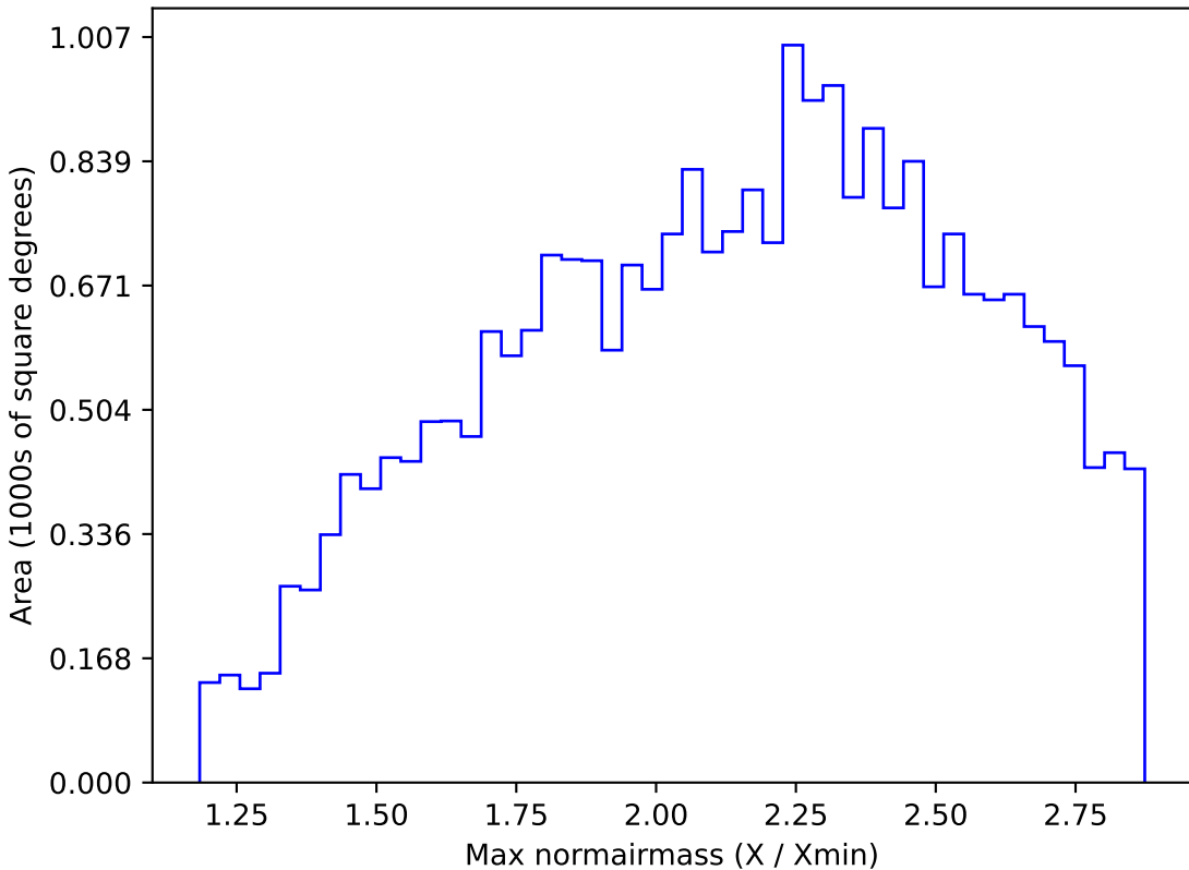
smc_lmc_v3.3_10yrs All sky i band: Max normairmass
