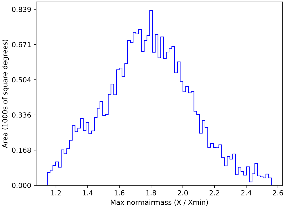
smc_lmc_v3.3_10yrs All sky g band: Max normairmass
