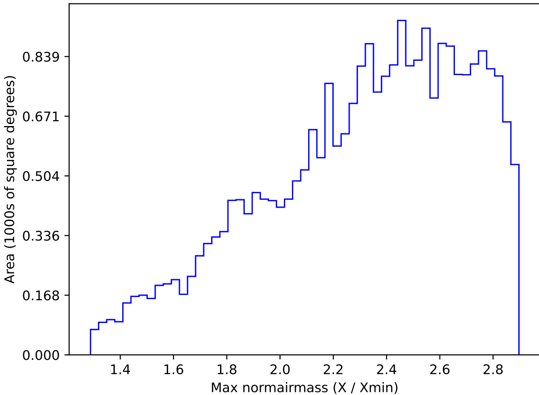
smc_lmc_v3.3_10yrs All sky all bands: Max normairmass
