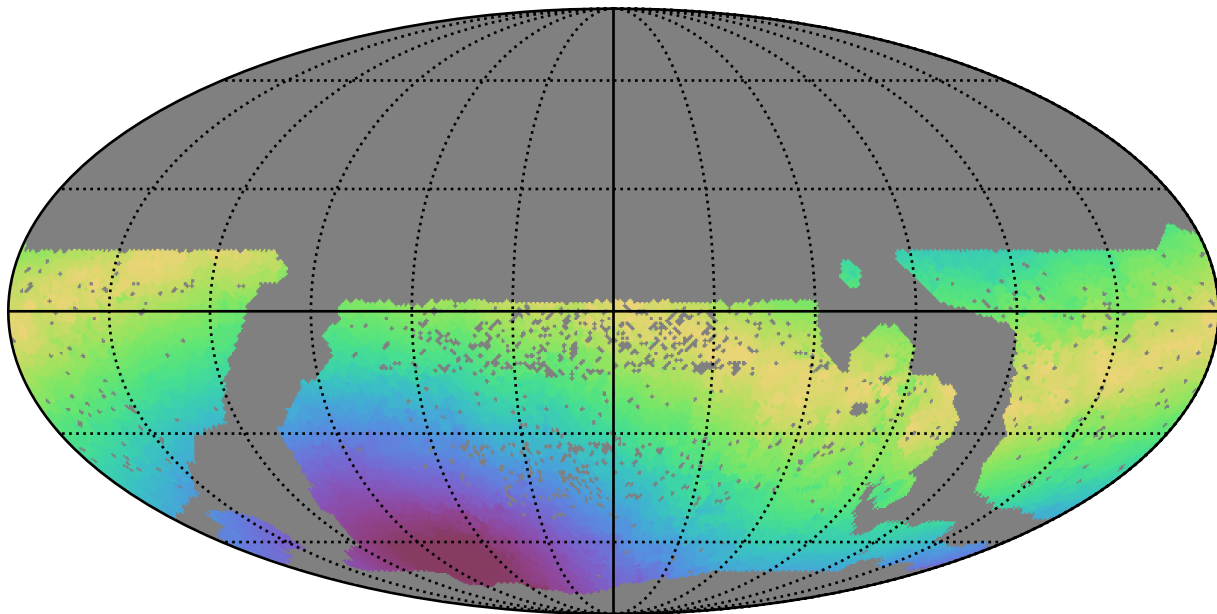
smc_lmc_v3.3_10yrs WFD u band: Max moonDistance
