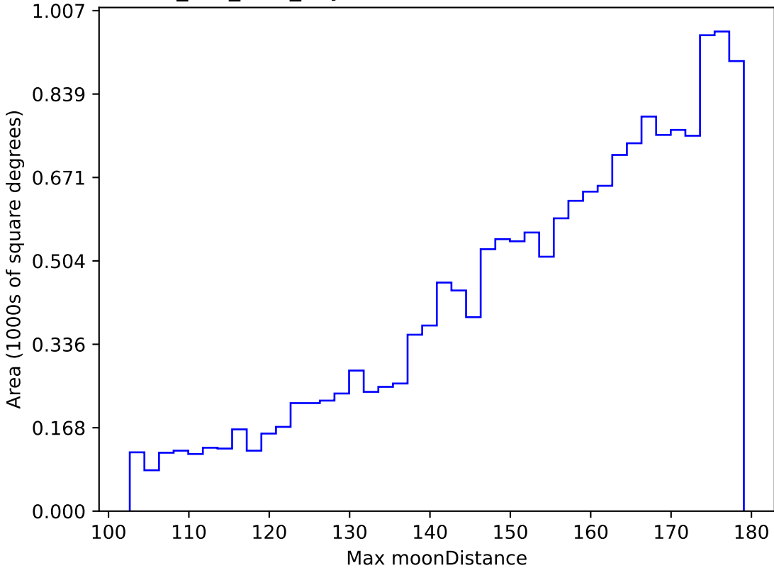
smc_lmc_v3.3_10yrs WFD u band: Max moonDistance
