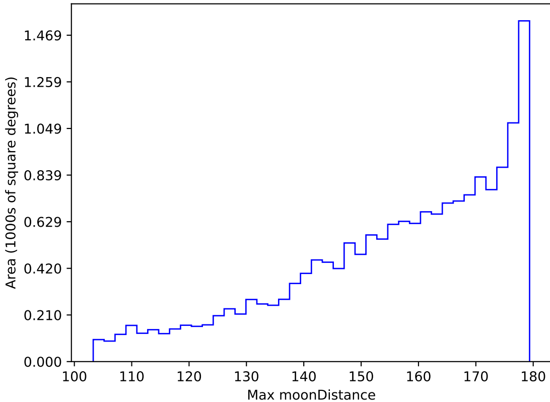
smc_lmc_v3.3_10yrs WFD r band: Max moonDistance
