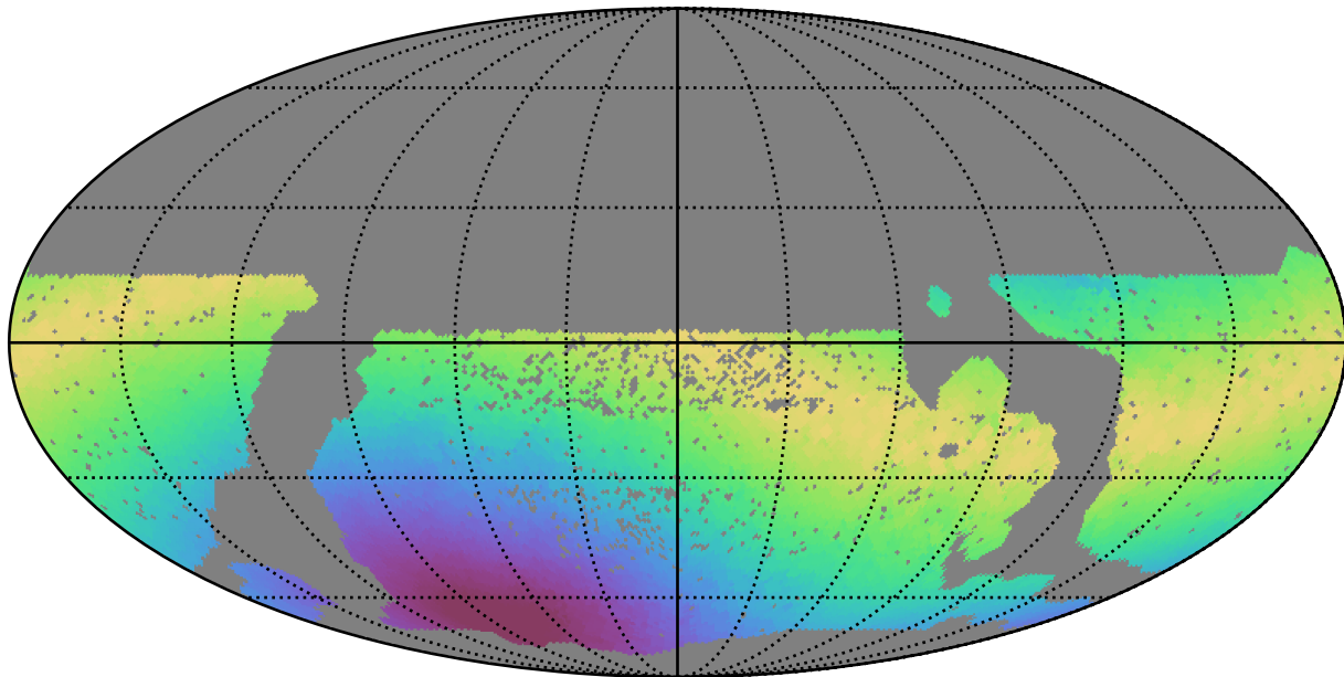
smc_lmc_v3.3_10yrs WFD i band: Max moonDistance
