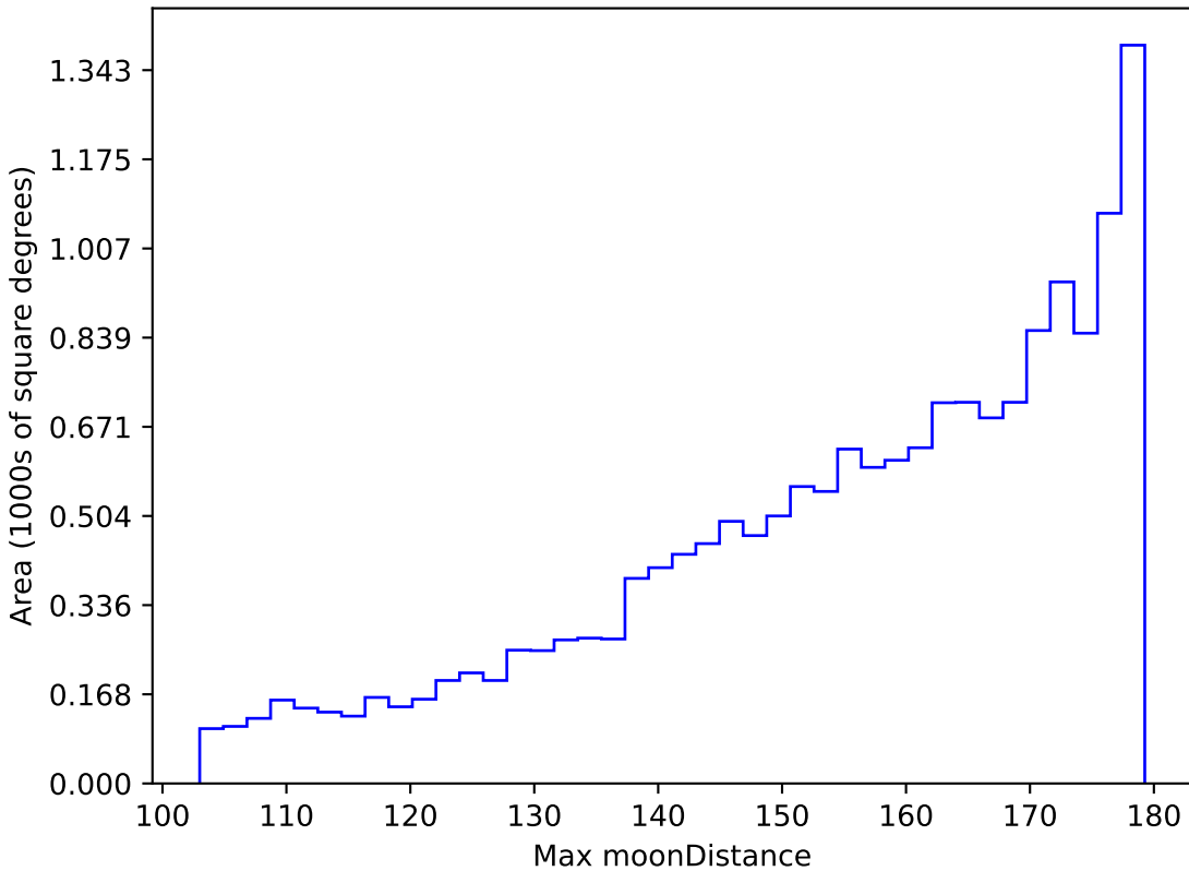
smc_lmc_v3.3_10yrs WFD i band: Max moonDistance
