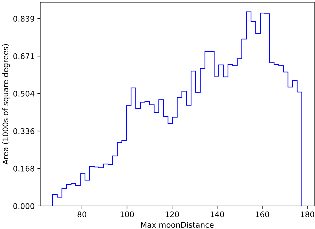
smc_lmc_v3.3_10yrs All sky y band: Max moonDistance
