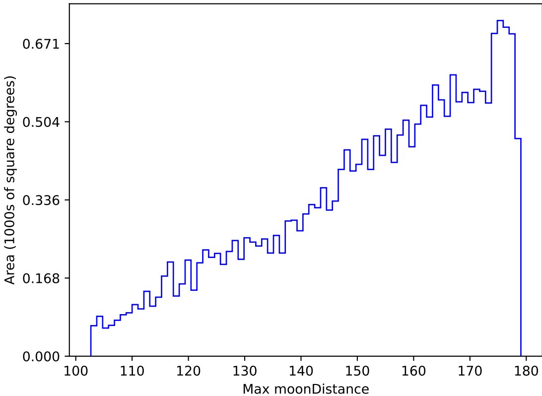
smc_lmc_v3.3_10yrs All sky u band: Max moonDistance
