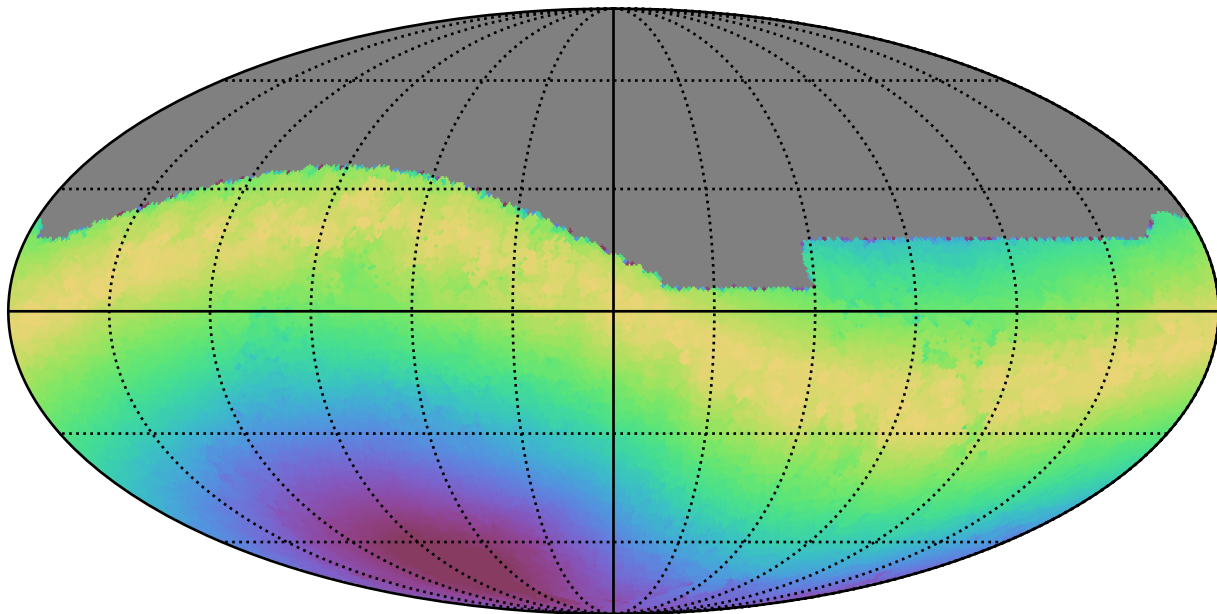
smc_lmc_v3.3_10yrs All sky r band: Max moonDistance
