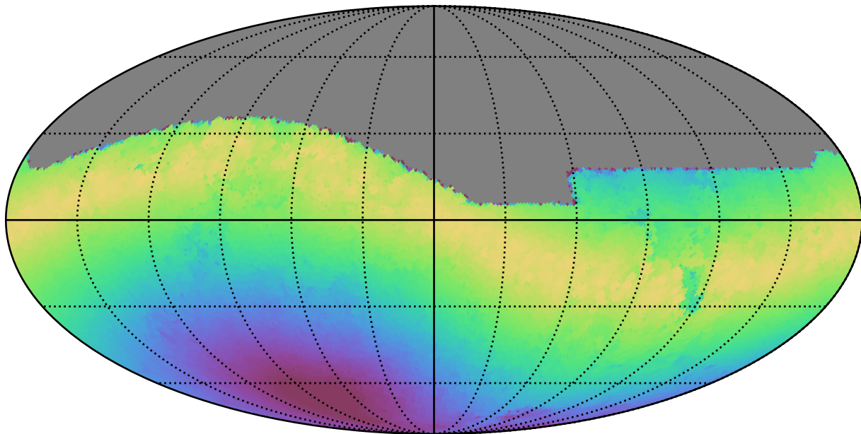
smc_lmc_v3.3_10yrs All sky i band: Max moonDistance
