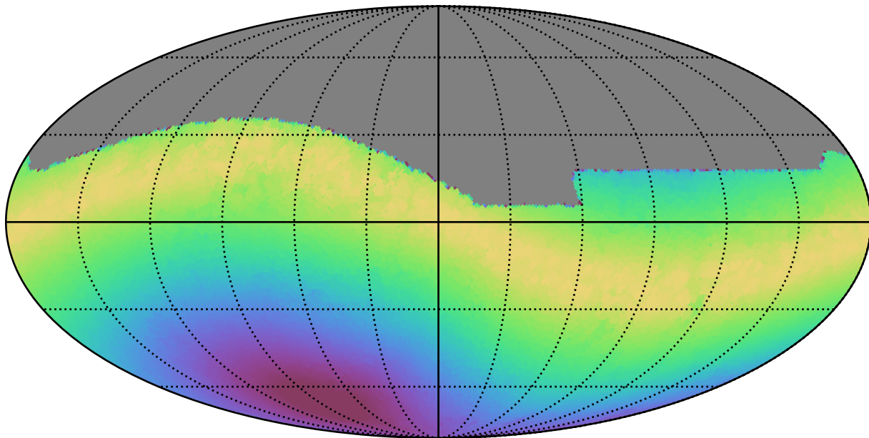
smc_lmc_v3.3_10yrs All sky all bands: Max moonDistance
