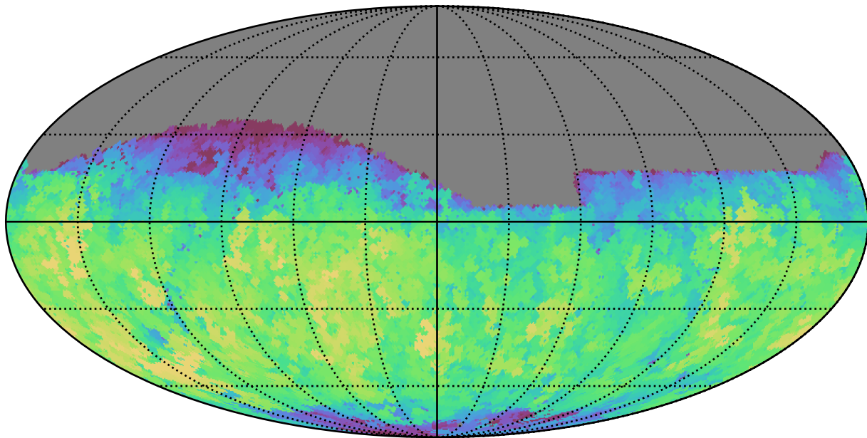
smc_lmc_v3.3_10yrs Yr 1 z band: Max fiveSigmaDepth
