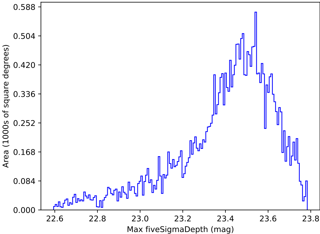
smc_lmc_v3.3_10yrs Yr 1 z band: Max fiveSigmaDepth
