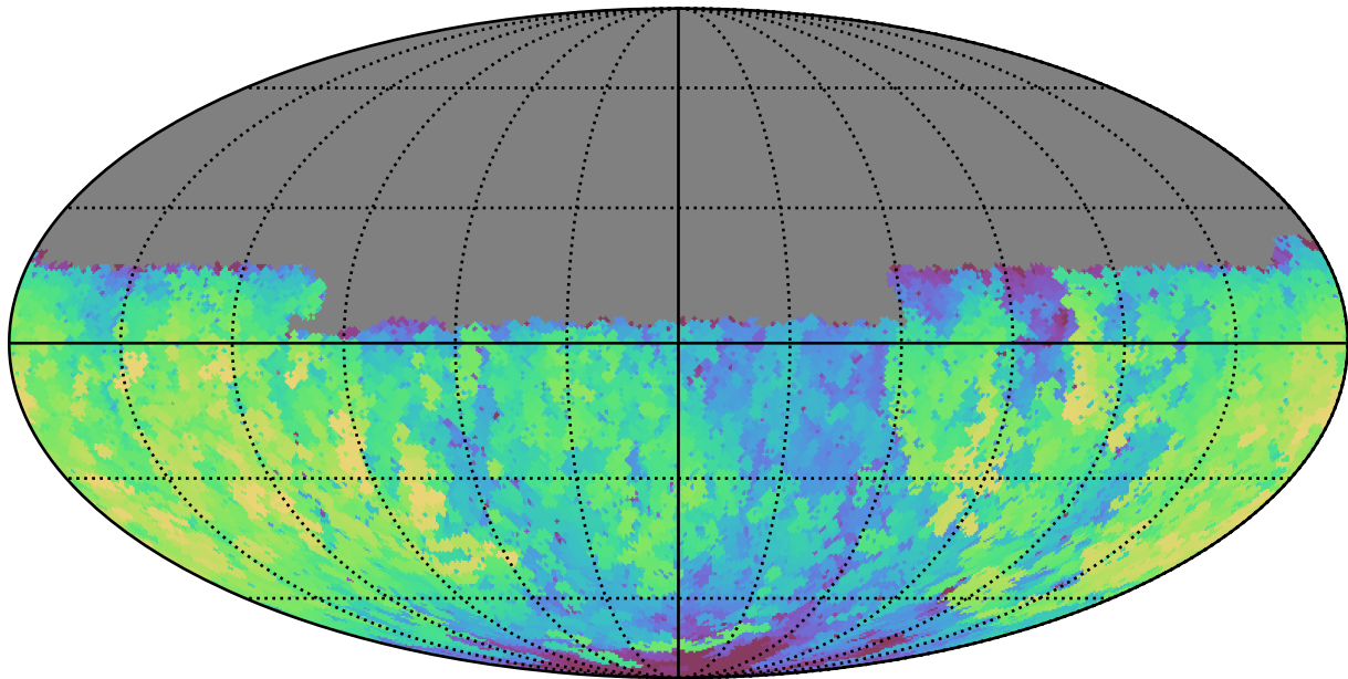
smc_lmc_v3.3_10yrs Yr 1 u band: Max fiveSigmaDepth
