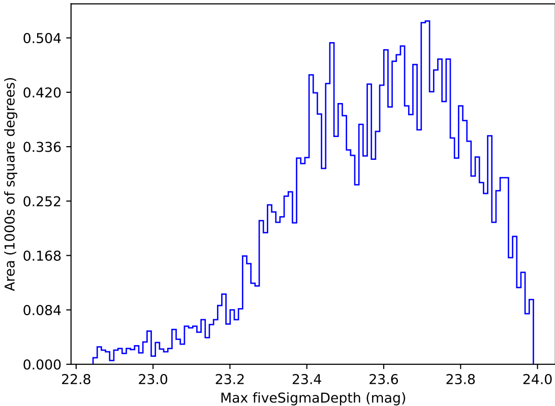
smc_lmc_v3.3_10yrs Yr 1 u band: Max fiveSigmaDepth
