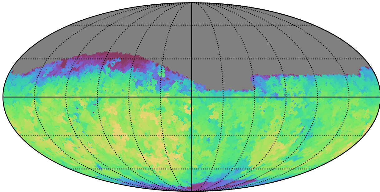
smc_lmc_v3.3_10yrs Yr 1 r band: Max fiveSigmaDepth
