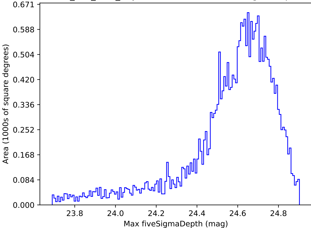
smc_lmc_v3.3_10yrs Yr 1 r band: Max fiveSigmaDepth
