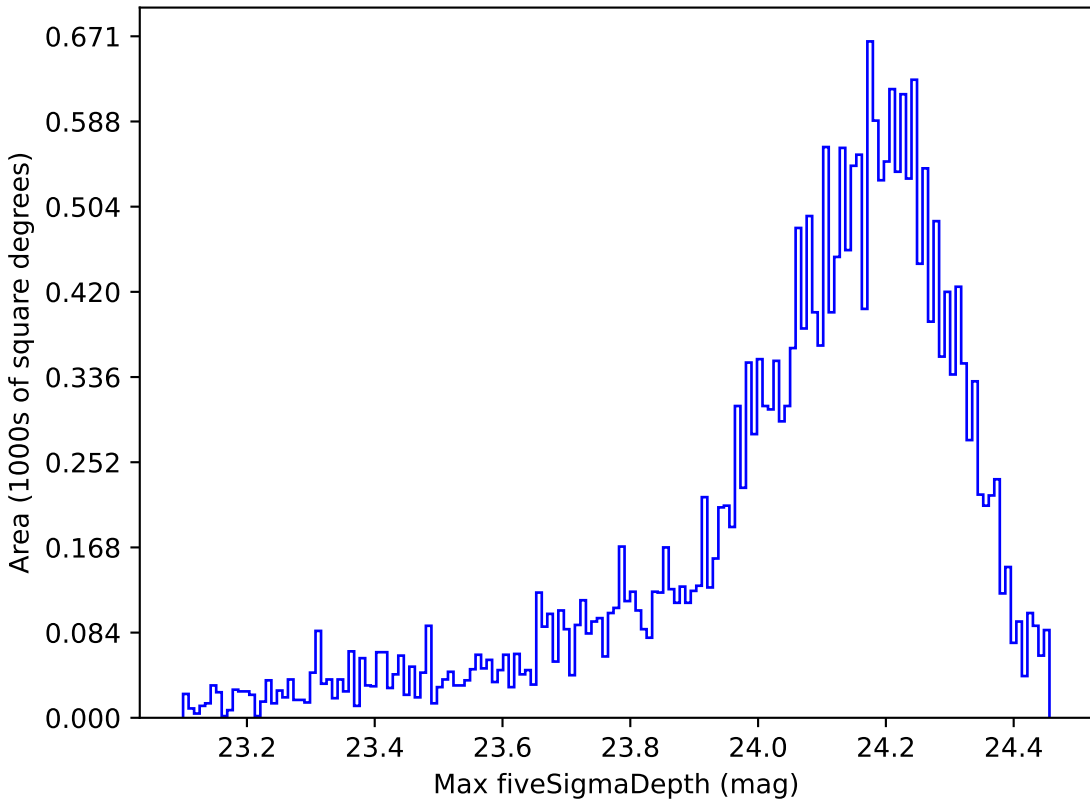
smc_lmc_v3.3_10yrs Yr 1 i band: Max fiveSigmaDepth
