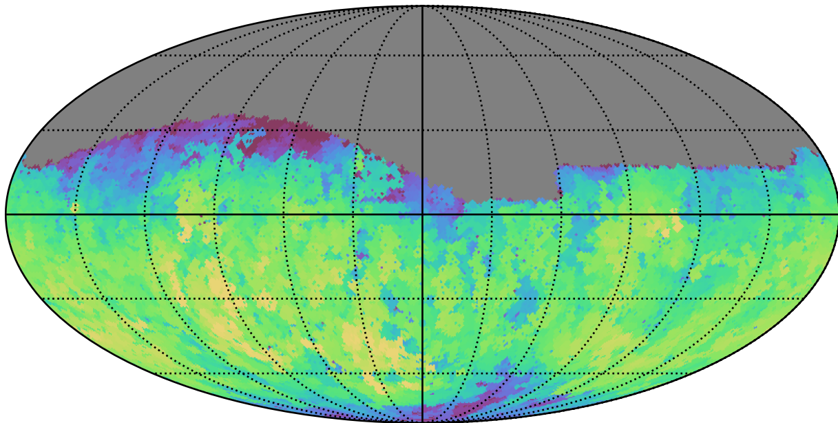
smc_lmc_v3.3_10yrs Yr 1 g band: Max fiveSigmaDepth
