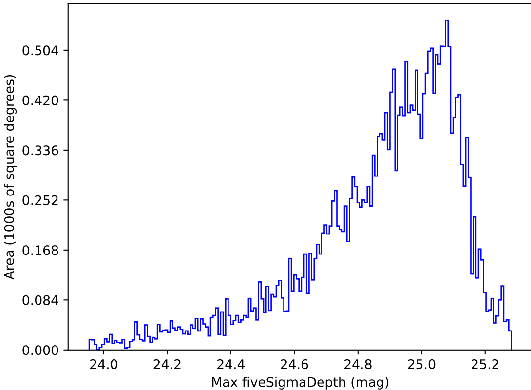
smc_lmc_v3.3_10yrs Yr 1 g band: Max fiveSigmaDepth
