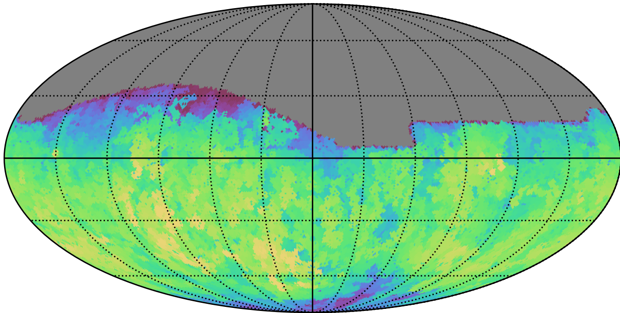
smc_lmc_v3.3_10yrs Yr 1 all bands: Max fiveSigmaDepth
