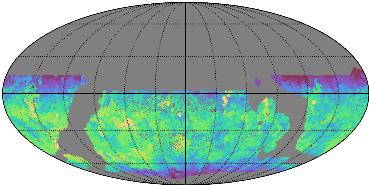
smc_lmc_v3.3_10yrs WFD z band: Max fiveSigmaDepth
