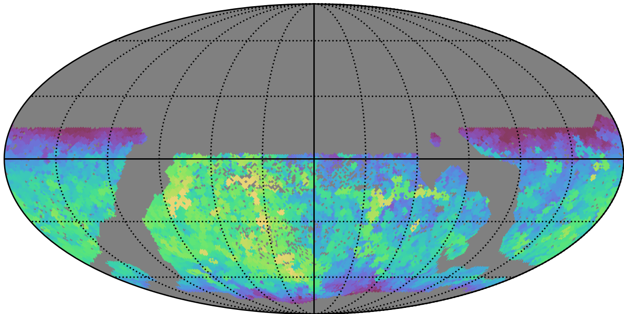
smc_lmc_v3.3_10yrs WFD r band: Max fiveSigmaDepth
