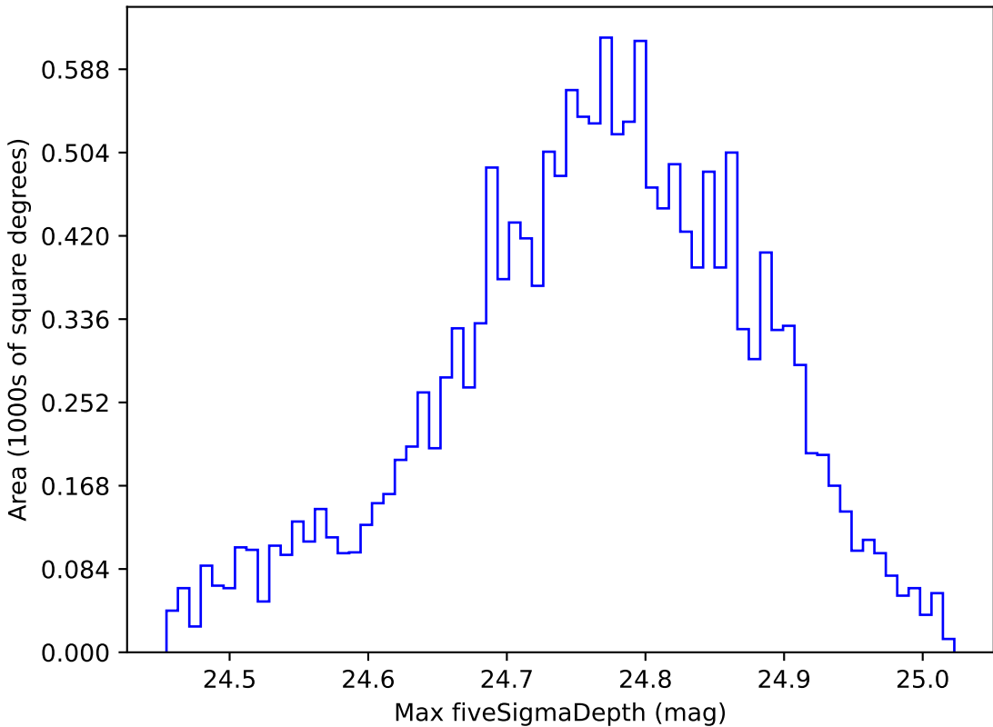
smc_lmc_v3.3_10yrs WFD r band: Max fiveSigmaDepth
