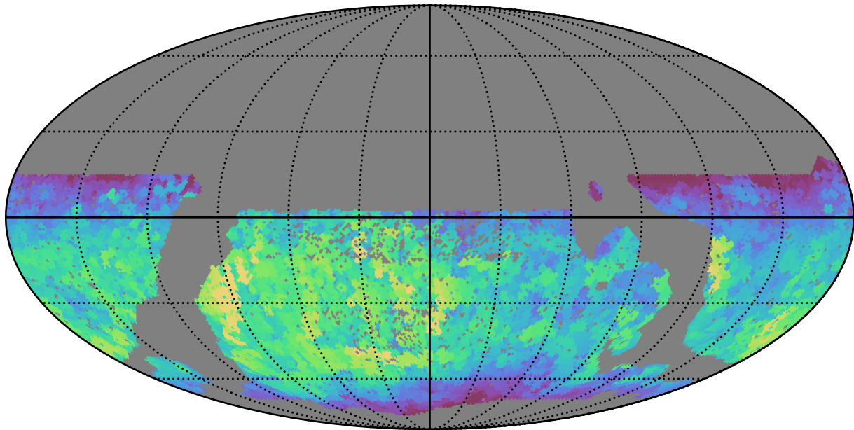
smc_lmc_v3.3_10yrs WFD i band: Max fiveSigmaDepth
