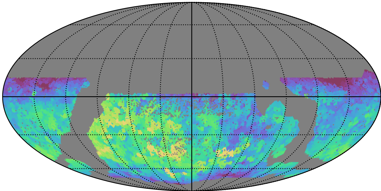
smc_lmc_v3.3_10yrs WFD g band: Max fiveSigmaDepth
