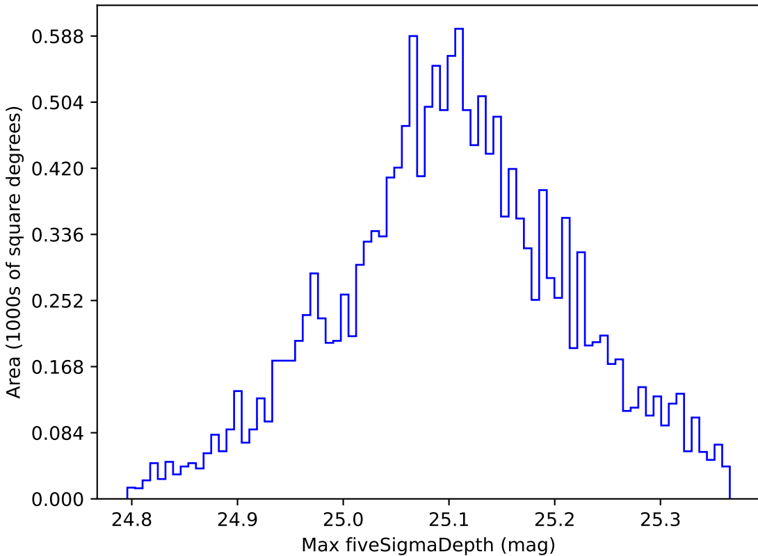
smc_lmc_v3.3_10yrs WFD g band: Max fiveSigmaDepth
