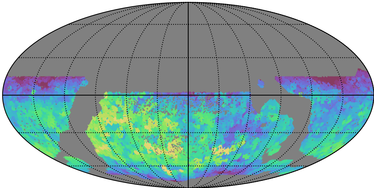
smc_lmc_v3.3_10yrs WFD all bands: Max fiveSigmaDepth
