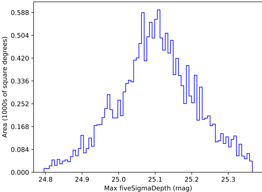
smc_lmc_v3.3_10yrs WFD all bands: Max fiveSigmaDepth
