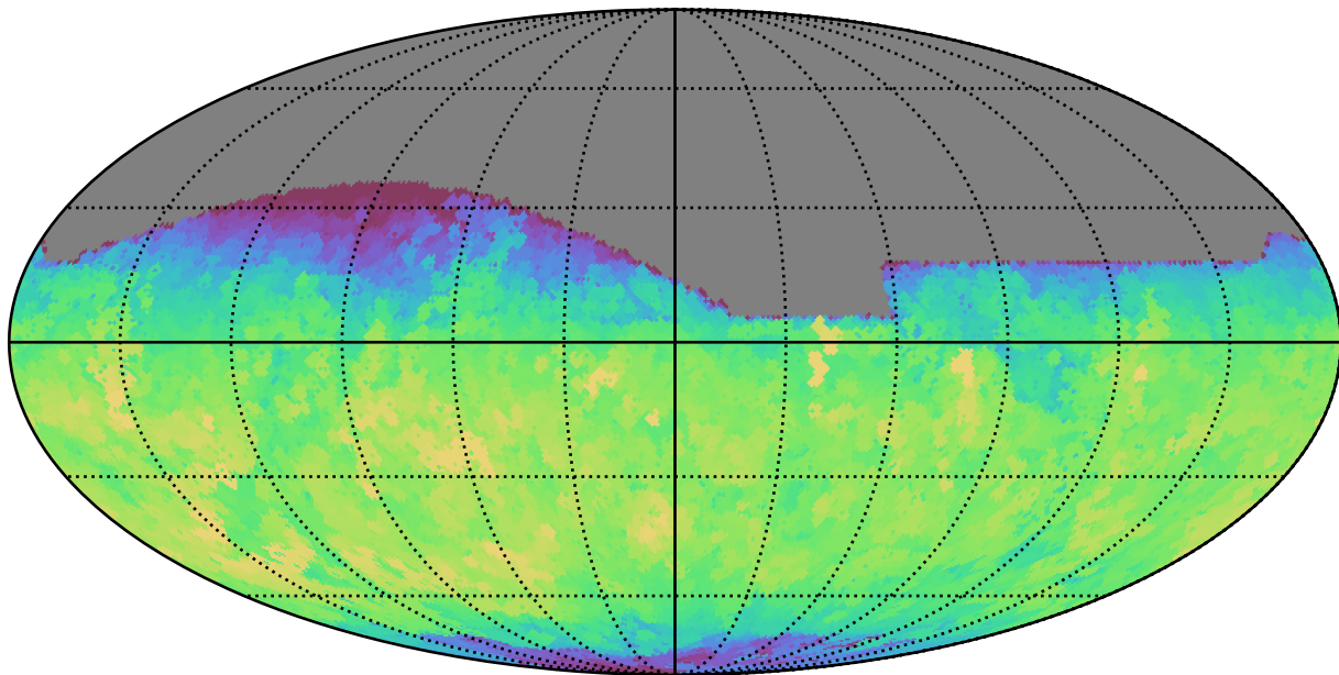
smc_lmc_v3.3_10yrs All sky z band: Max fiveSigmaDepth
