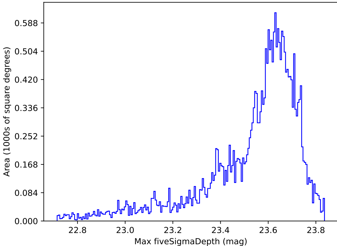
smc_lmc_v3.3_10yrs All sky z band: Max fiveSigmaDepth
