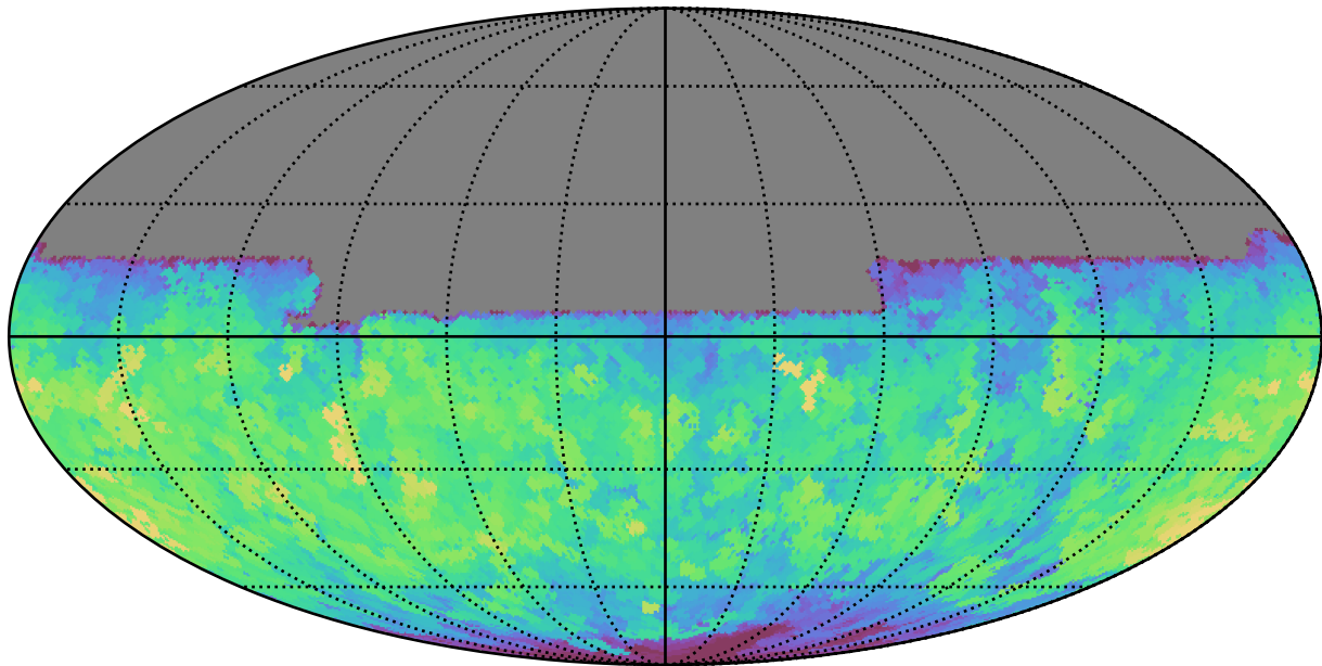
smc_lmc_v3.3_10yrs All sky u band: Max fiveSigmaDepth
