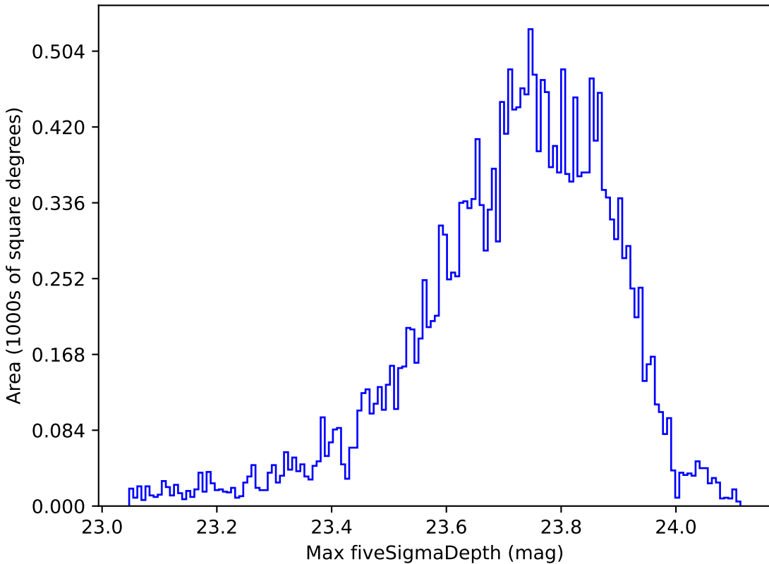
smc_lmc_v3.3_10yrs All sky u band: Max fiveSigmaDepth
