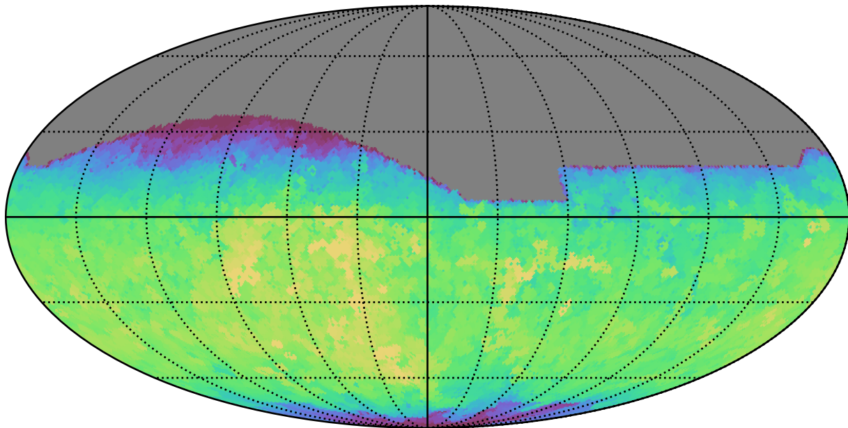
smc_lmc_v3.3_10yrs All sky r band: Max fiveSigmaDepth
