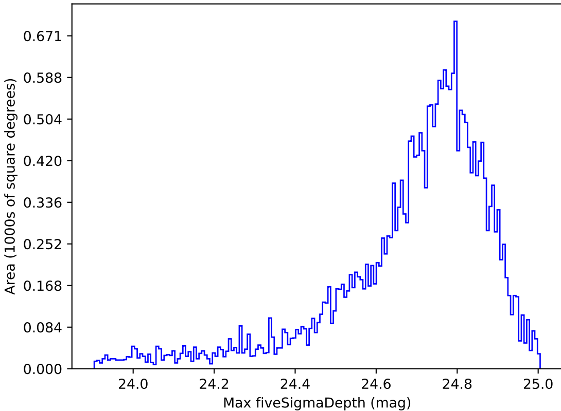
smc_lmc_v3.3_10yrs All sky r band: Max fiveSigmaDepth
