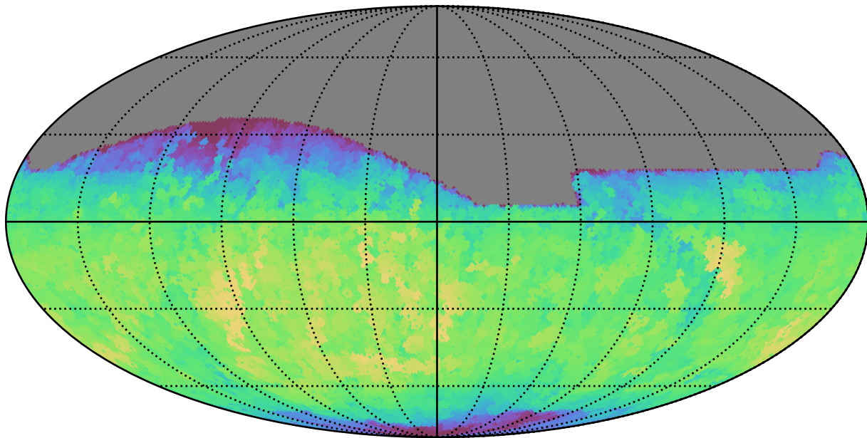
smc_lmc_v3.3_10yrs All sky i band: Max fiveSigmaDepth
