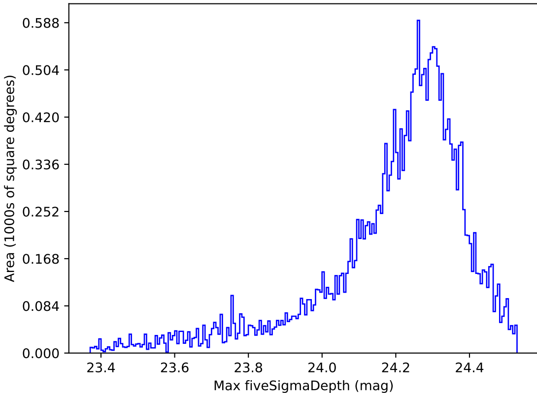
smc_lmc_v3.3_10yrs All sky i band: Max fiveSigmaDepth
