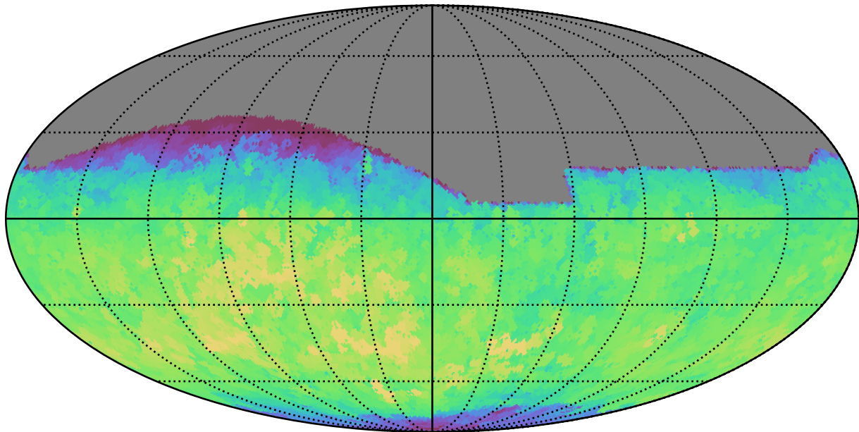
smc_lmc_v3.3_10yrs All sky g band: Max fiveSigmaDepth
