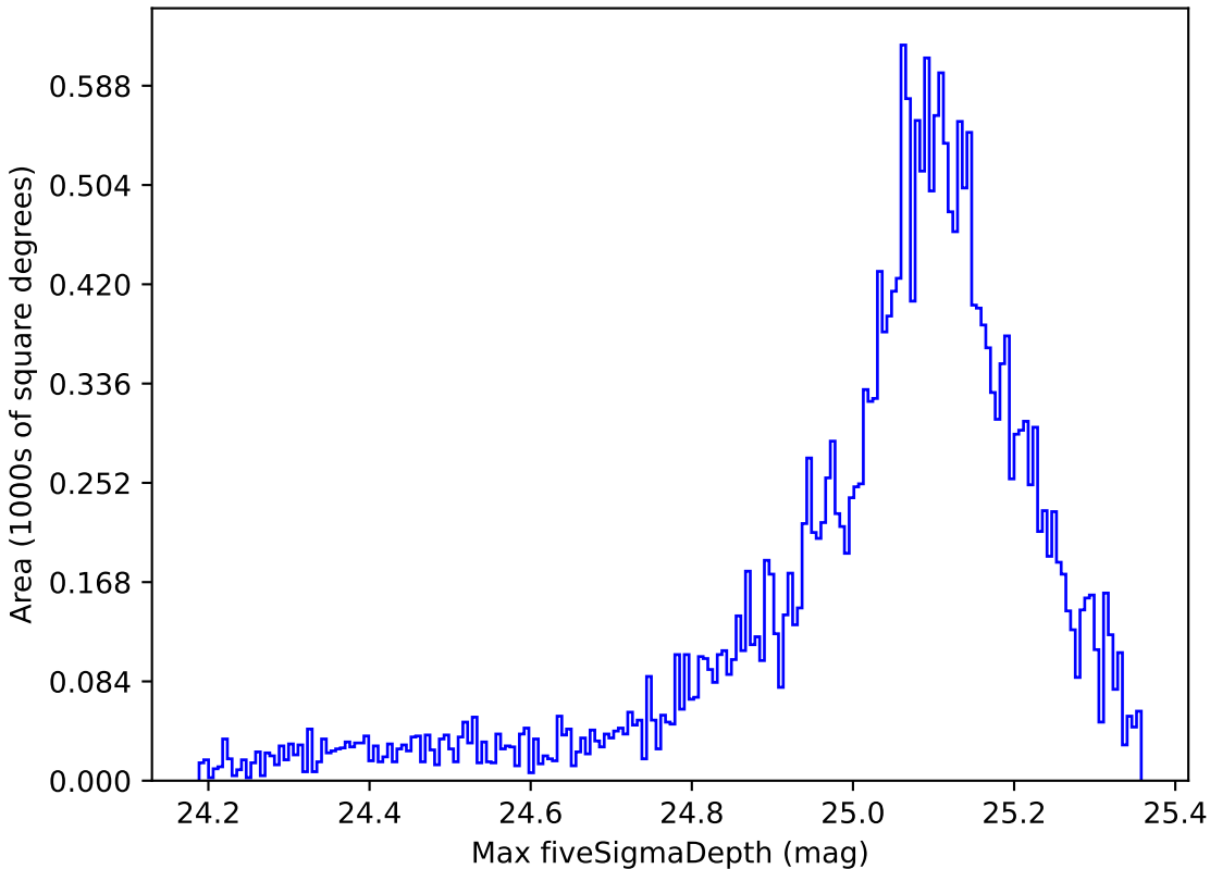
smc_lmc_v3.3_10yrs All sky g band: Max fiveSigmaDepth
