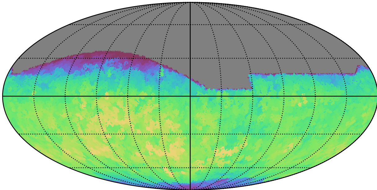
smc_lmc_v3.3_10yrs All sky all bands: Max fiveSigmaDepth
