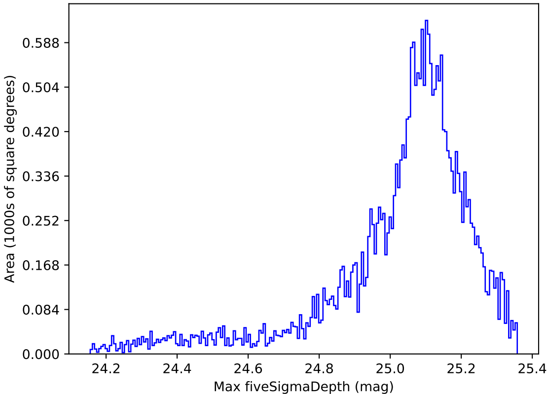
smc_lmc_v3.3_10yrs All sky all bands: Max fiveSigmaDepth
