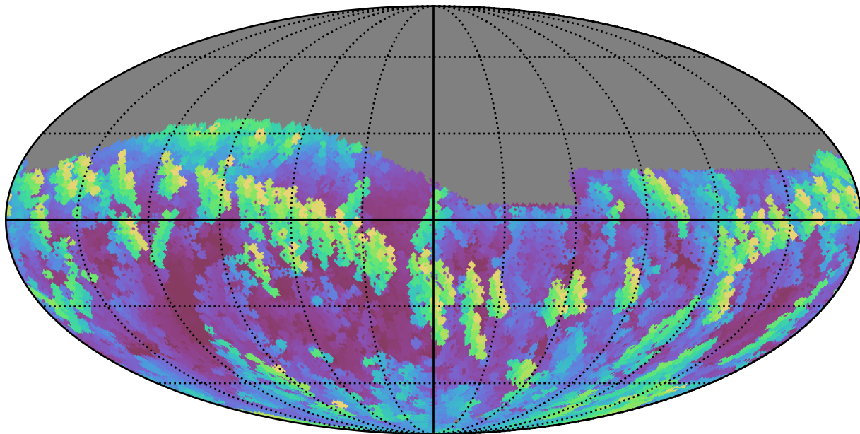
smc_lmc_v3.3_10yrs Yr 1 z band: Max airmass
