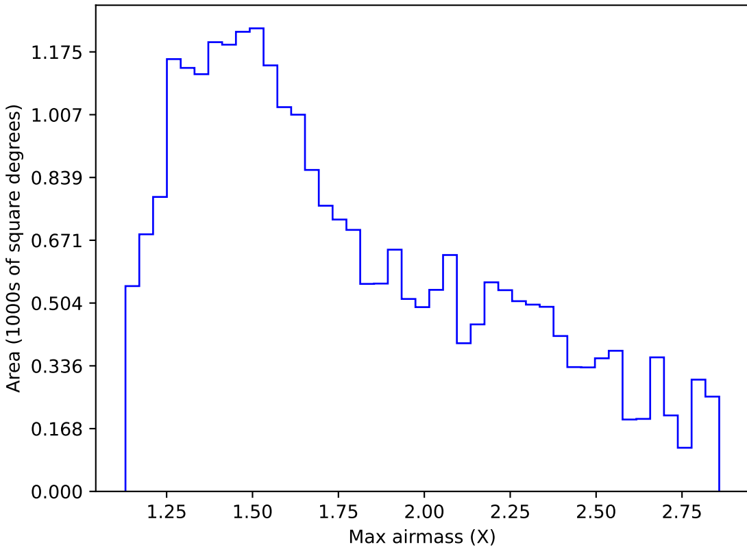
smc_lmc_v3.3_10yrs Yr 1 z band: Max airmass
