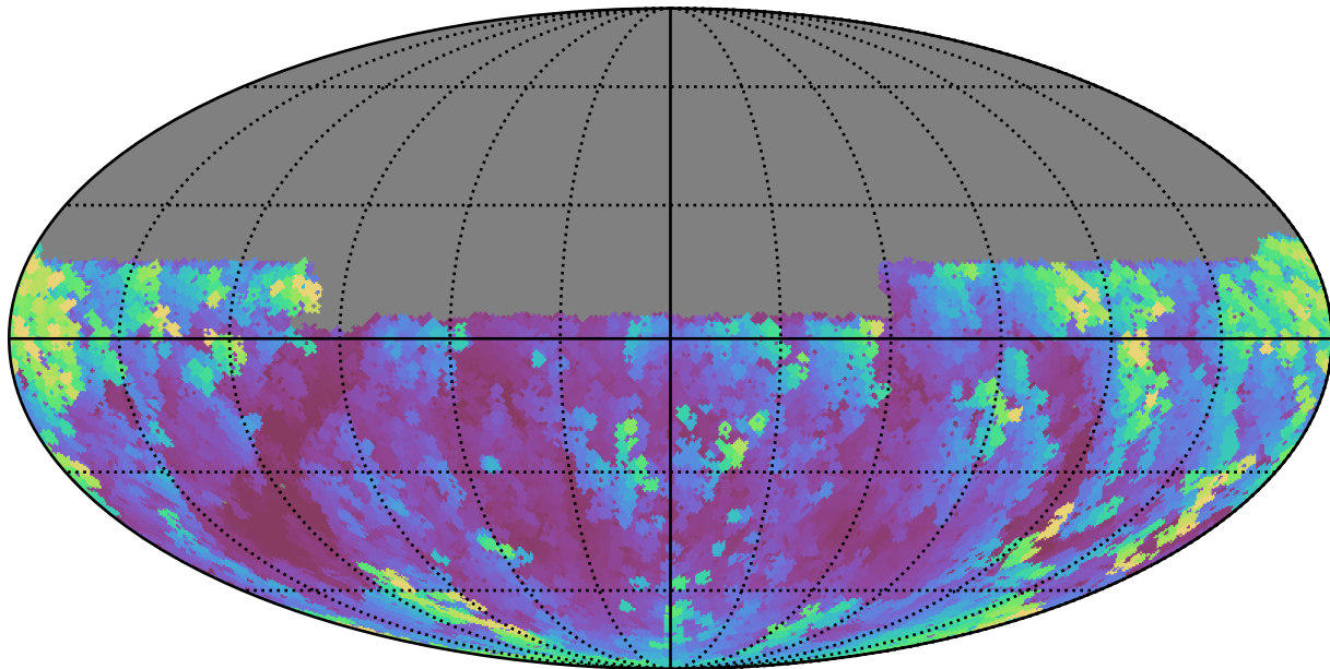
smc_lmc_v3.3_10yrs Yr 1 y band: Max airmass
