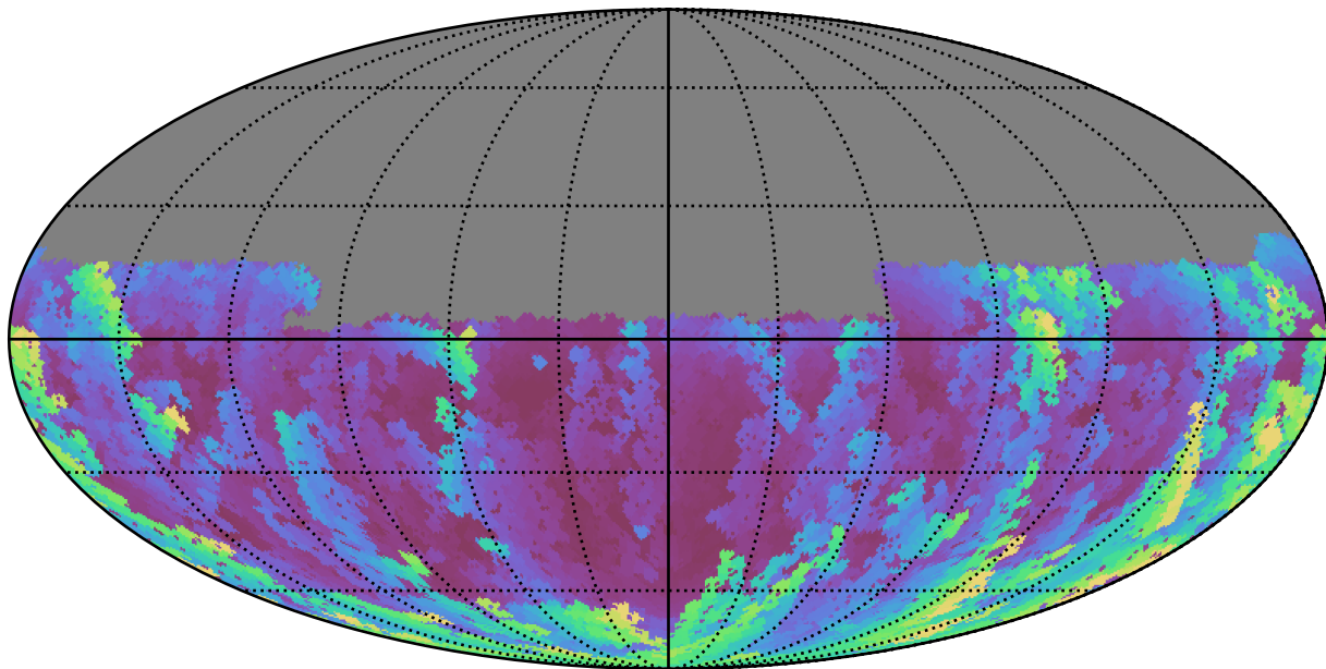
smc_lmc_v3.3_10yrs Yr 1 u band: Max airmass
