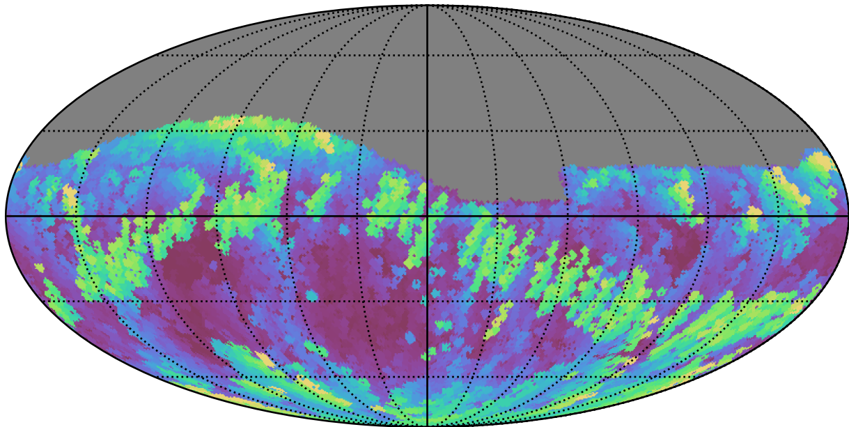
smc_lmc_v3.3_10yrs Yr 1 r band: Max airmass
